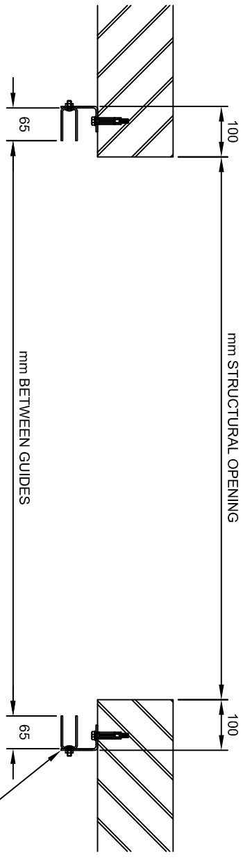
Plan At Guide Level
